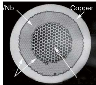
CuNi-NbTi Reinforced
